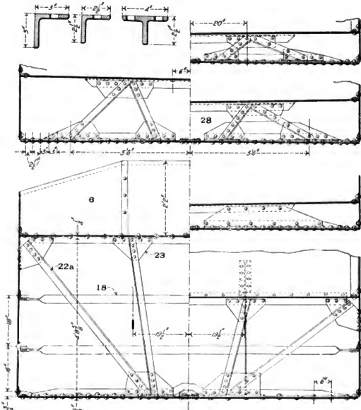
Figs. 4094-4101. Cross-Sections of 5,500-Gallon Tender Tank for Atlantic (4-4-2) Locomotive. P. R. R.
